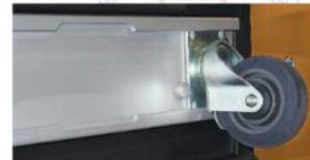
Slide Mount Casters with 'spring-out' Position Stops
